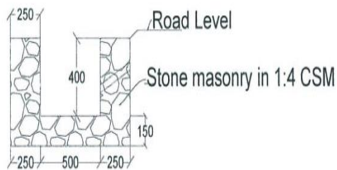
Drain Type - I
