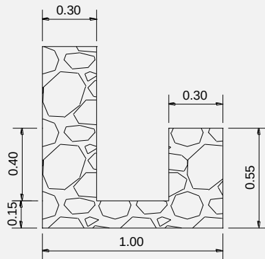
Sketch Item servisu Stone Masonry Retaining wall
