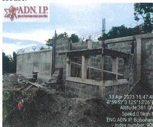
Foto: Servisu pengecoran column Guard House.
